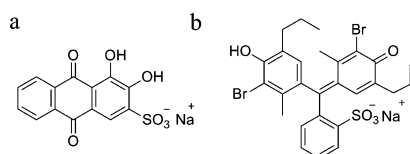
Figure 4. Chemical structures of anionic dyes: (a) ARS (b) BTB.
